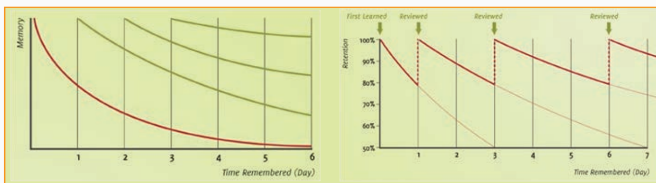
Forgetting curve
